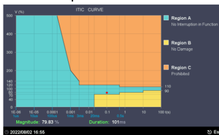
ITIC Plot
