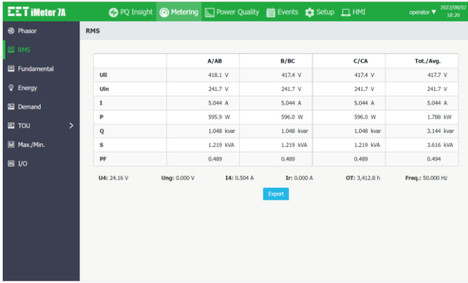
RMS Metering
